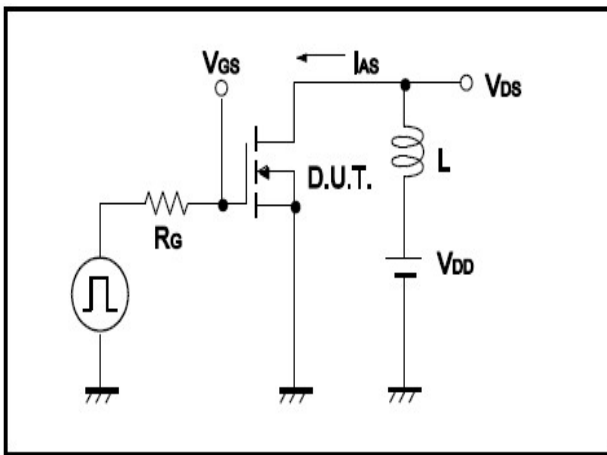
Fig.16 Avalanche Measurement Circuit
