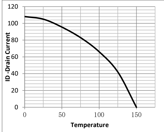
Fig.8 ID-Junction Temperature
